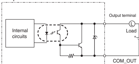
Output Circuit
